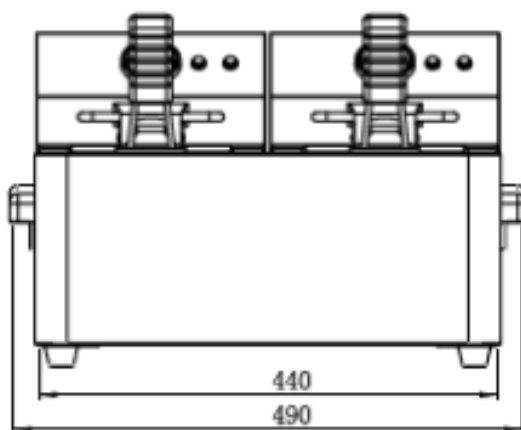
VISTA FRONTAL Front View
